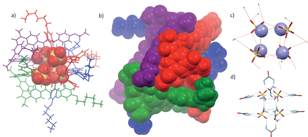
Figure 3. a) Representation of the complex [(\text{SO}_4^{2-})_4 \cdot \text{H}4]^{4-} showing the encapsulation of the four sulfate anions (given in space-filling representation) inside the capsule formed by four molecules of \text{H}4^+ (stick representation; a different color is used per unit of \text{H}4^+ ). b) Space-filling representation of the complex [(\text{SO}_4^{2-})_4 \cdot \text{H}4]^{4-} when viewed down the c^* crystallographic axis showing the arrangement and packing of the \text{H}4 self-assembled structure. c) and d) The hydrogen-bonding network within the cavity. The blue spheres in (c) represent protonated amino moieties.
